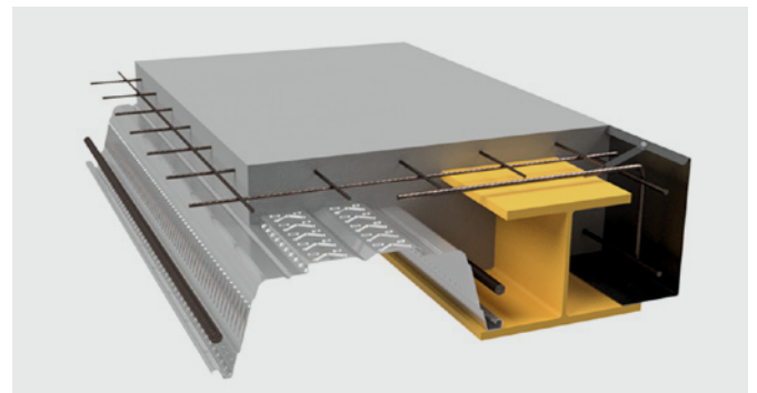
Figure F.3.5.1 Fielders SlimFlor®
