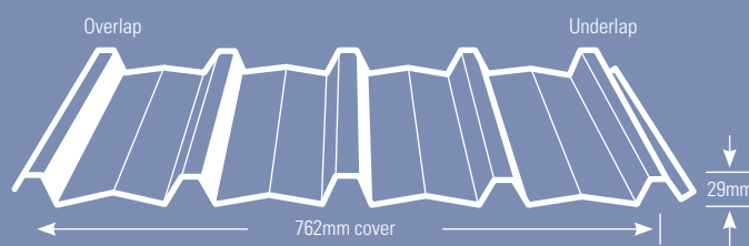
Figure 1: TL-5 Profile
